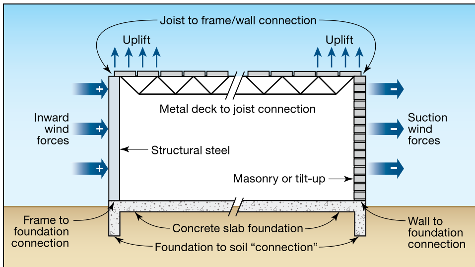
Figure B3-5. Critical connections important for providing a continuous load path in a typical masonry, concrete, or metal-frame building wall (for clarity, concrete roof deck is not shown)
